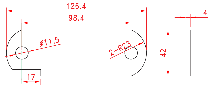
Retainer Bracket Gasket FUDU-DGE08040
